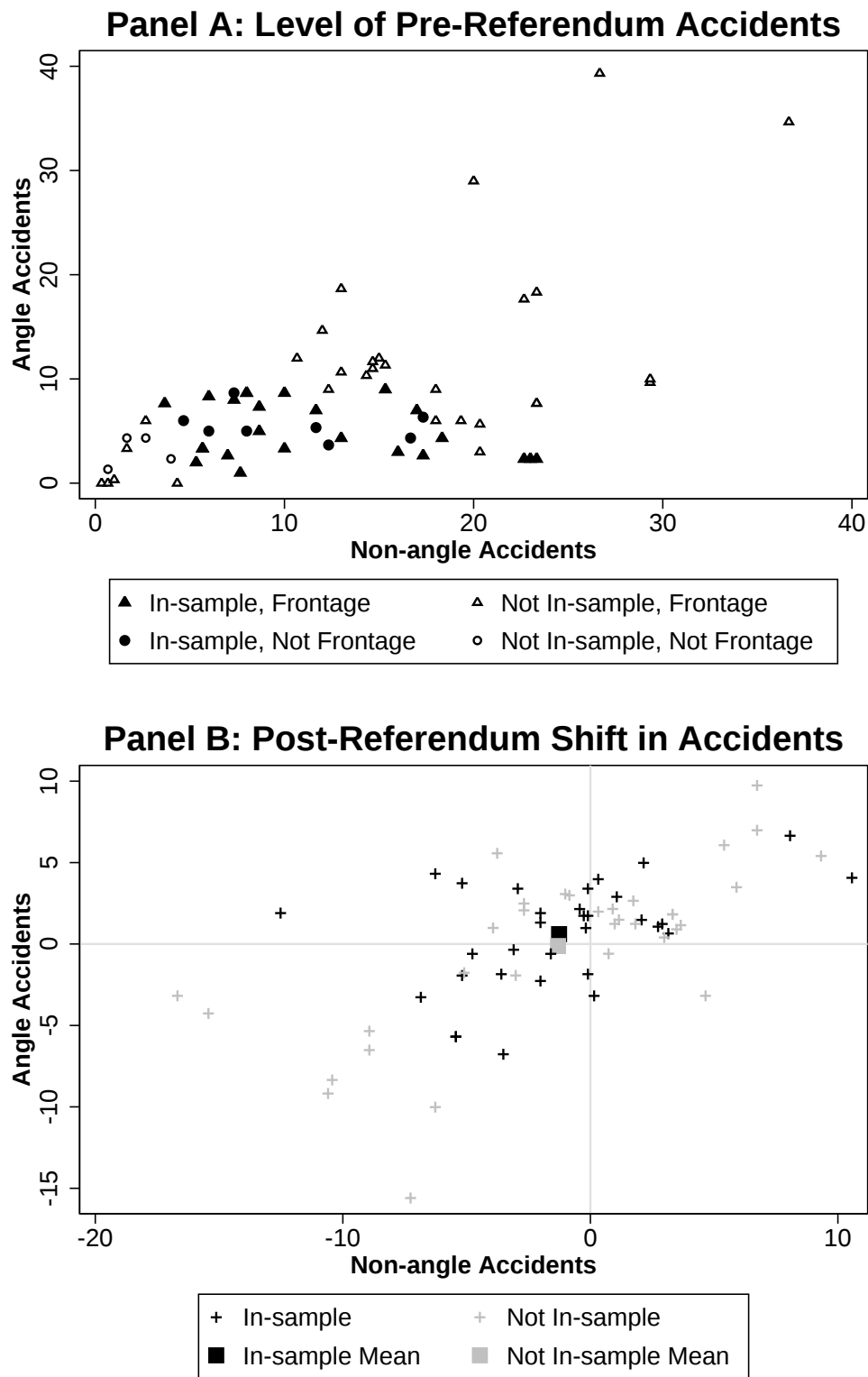
Figure 6: Angle and Non-angle Accidents by Camera Intersection
