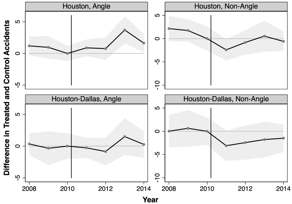
Figure 5: Angle and Non-angle Accident Trends for Treatment and Control Intersections
