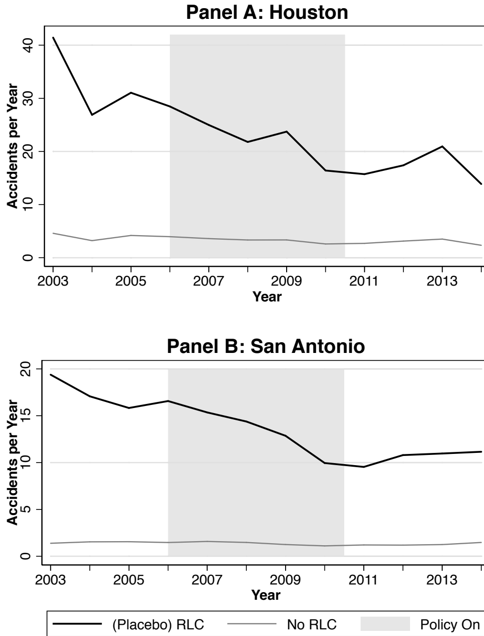
Figure 4: Intersection Vehicle Accident Trends
